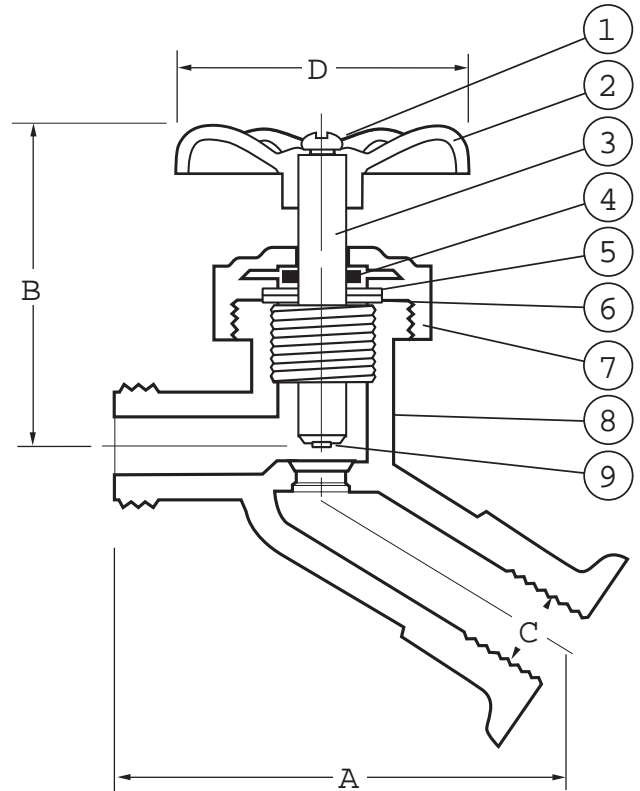
Pictured Model T-628 Cut-away
