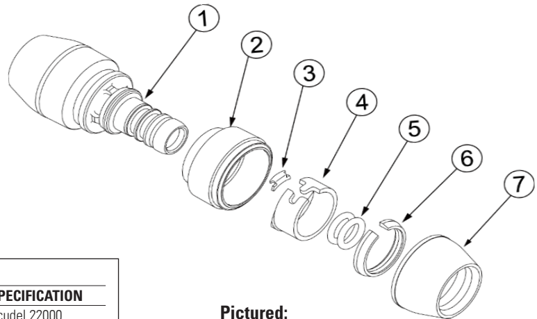
Pictured: SmartClick Connection Exploded View
